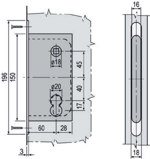
Drilling diagram
