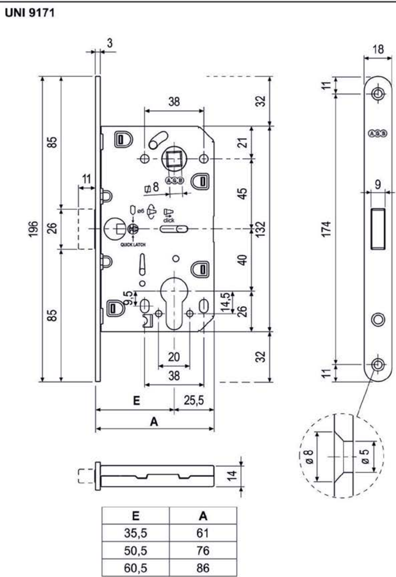
Drilling diagram
