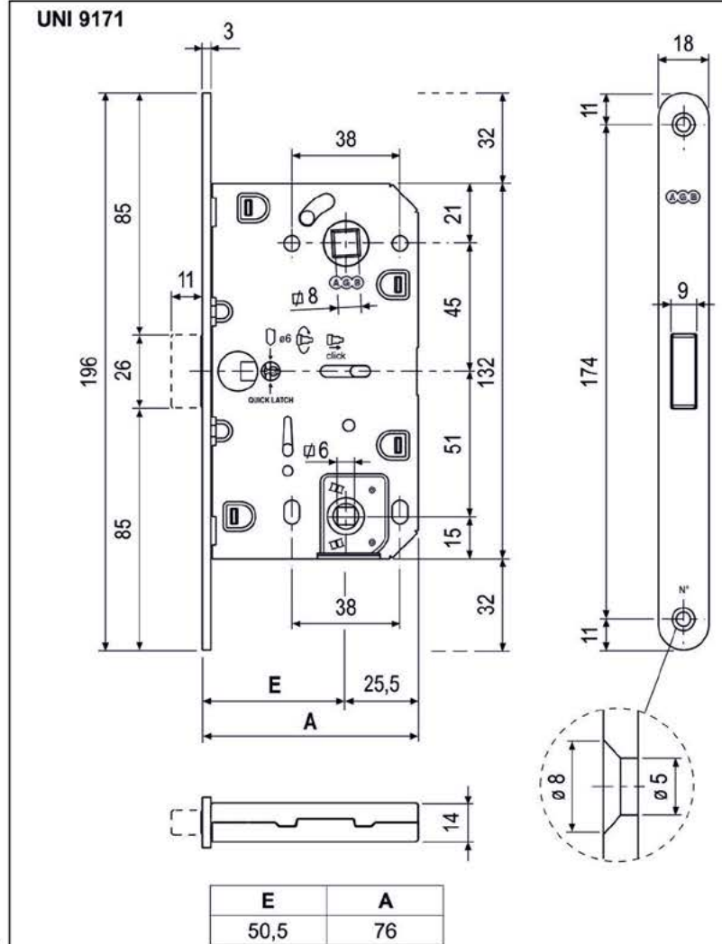
Drilling diagram
