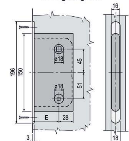
Drilling diagram
