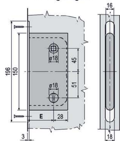
Drilling diagram
